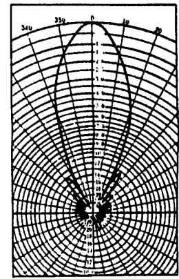
Vertical Polarization, H-plane
